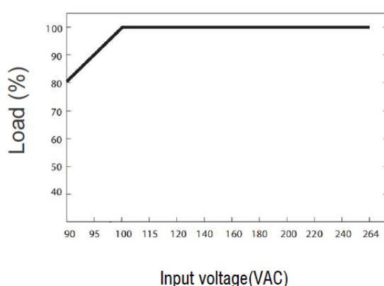
■ Minus output and input voltage curves
